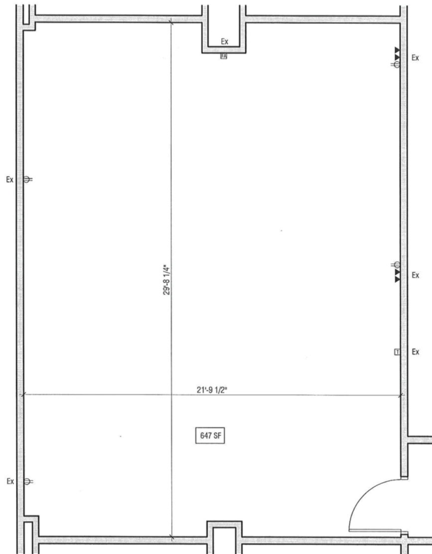
Suite 109 Floorplan
